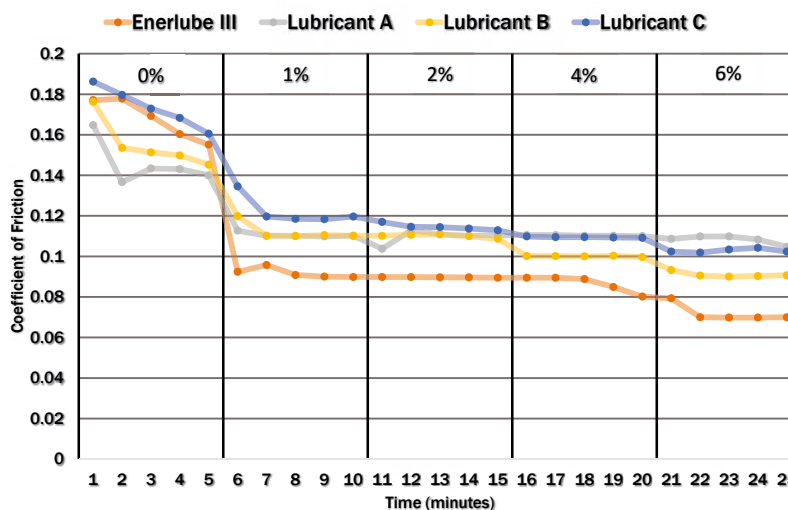
EnerLube III Coefficient of Friction Comparison 20%/wt Sodium Chloride Brine
